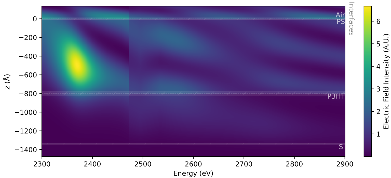
X-ray Electric Field Intensity at \theta=0.55^\circ
